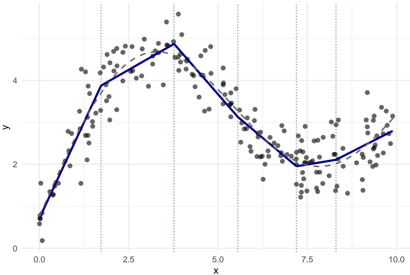
Linear regression spline (K = 5 knots, tuned by 5-fold CV)
