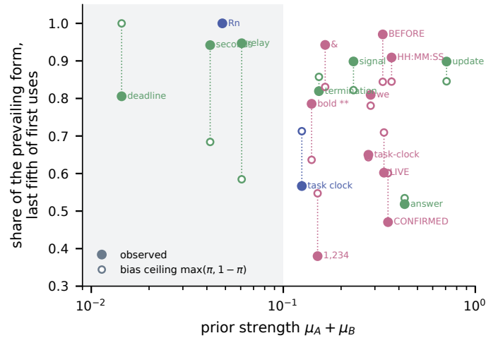
Figure S7: Weak priors settle by history, strong priors sit where the prior puts them. For each kept convention, the share of the prevailing form among the last fifth of first uses (filled) and the prior ceiling \max(\pi, 1 - \pi) implied by the fitted prior probabilities (open), against the prior strength \mu_A + \mu_B . The shaded region marks priors below 0.1.
