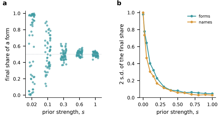
Figure S11: Who wrote first decides, or not. (a) Final share of one form over all uses of a run, for a convention read from the page with \pi = 0.5 , one dot per run, 50 runs at each of five prior strengths. (b) Twice the standard deviation of the final share across the 50 runs, against the prior strength, for a convention read from the page (teal) and a name feature read from the agents in view (amber).
