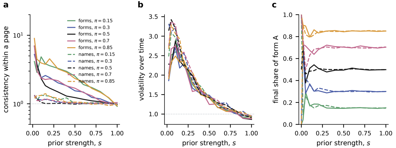
Figure S12: The strength of the prior orders the collective statistics, its direction sets which form wins. Median over 50 runs of (a) the co-occurrence ratio of the minority form, same page over different pages, (b) the volatility of the share relative to binomial noise, and (c) the final share of form A, against the prior strength s , for five directions of the prior \pi = \mu_A/s . Solid lines, conventions read from the page; dashed lines, name features read from the agents in view.
