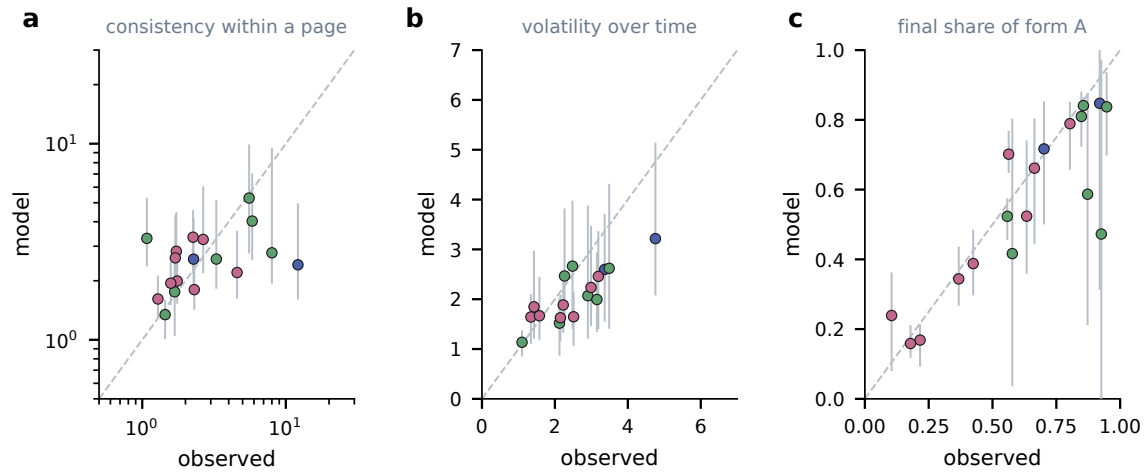
Figure S13: Each convention against the model run at its own fitted base probabilities. Median over 50 runs against the observed value, with the 10th to 90th percentile of the runs, for (a) the co-occurrence ratio, (b) the volatility relative to binomial noise, on first uses, and (c) the final share of form A. Colours give the class of the convention. The dashed line is equality.
