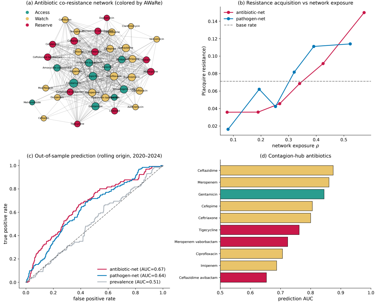
Figure 4: Prediction of resistance emergence from network exposure. (a) Antibiotic co-resistance network (NBI projection), nodes coloured by WHO AWaRe class, sized by degree. (b) Probability of acquiring a new resistance versus network-exposure \rho for the antibiotic and pathogen projections; dashed line is the base rate. (c) Out-of-sample ROC (pooled rolling-origin test): both network scores beat the prevalence baseline, which is uninformative under RCA. (d) Contagion-hub antibiotics: per-drug prediction AUC (colour = AWaRe class).
