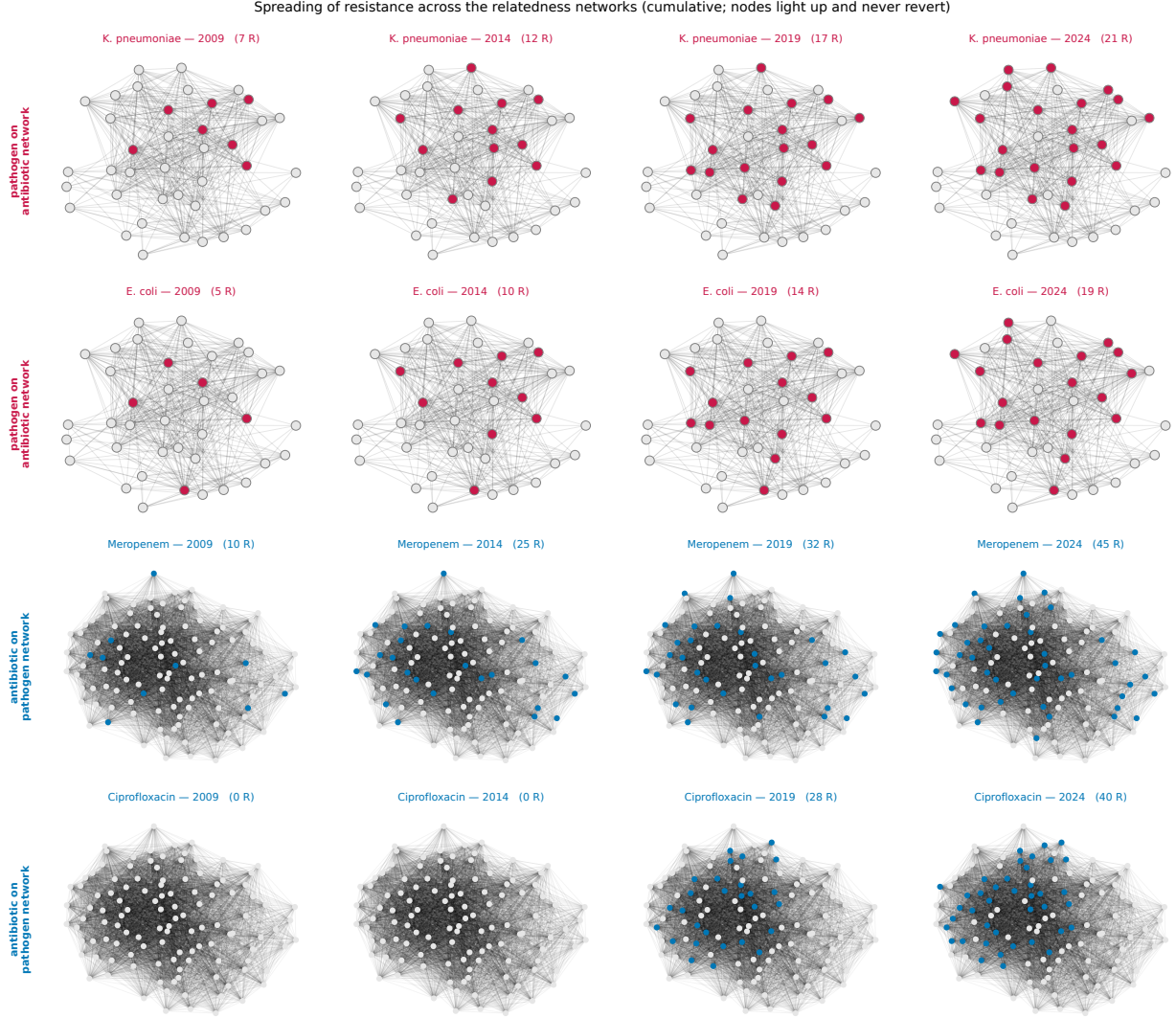
Figure 5: Spreading of resistance across the relatedness networks. Top two rows: two example pathogens ( K. pneumoniae , E. coli ) shown on the fixed antibiotic co-resistance network; a node is coloured when the pathogen has acquired RCA-resistance to that drug by the indicated year (cumulative, so nodes light up and never revert). Bottom two rows: two example antibiotics (meropenem, ciprofloxacin) shown on the pathogen relatedness network; a node is coloured when that species has become resistant. Resistance spreads to network-adjacent nodes rather than at random.
