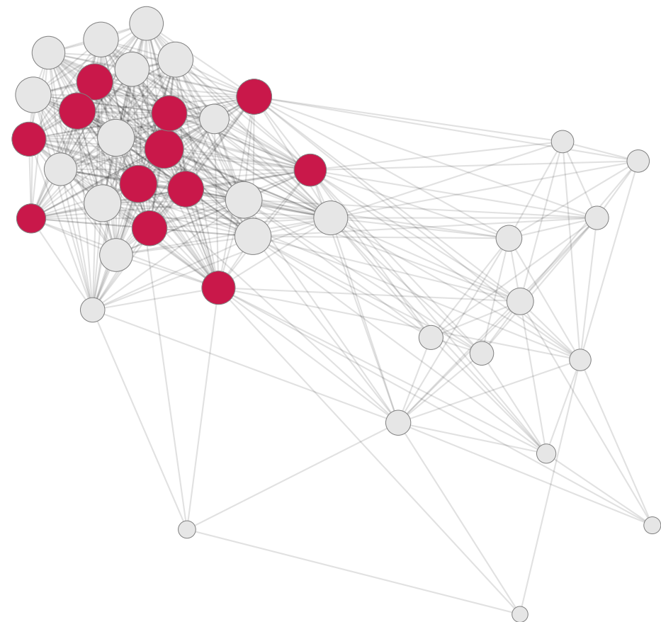
(b) K. pneumoniae — 2014 (12 drugs defeated)
