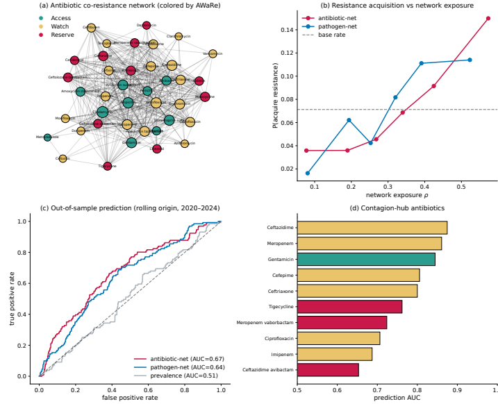
Figure 4: Prospective prioritisation. Panel (a) shows the antibiotic relatedness network; (b) shows next-year RCA-positive frequencies across exposure; (c) reports pooled prospective ROC curves; and (d) reports performance by antibiotic. Prediction uses raw co-occurrence weights; degree normalisation is used only for the network layout in (a). The event is a transition to RCA-positive status, not proof of biological acquisition.
