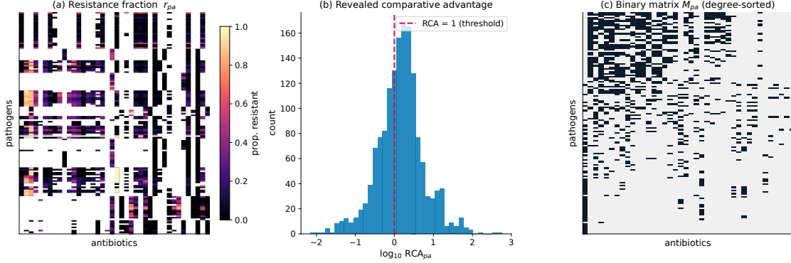
Figure 1: From surveillance counts to the bipartite network. Pooled resistance fractions (a) are normalised into RCA values (b) and thresholded at \text{RCA} = 1 to obtain M (c). RCA defines a comparative signal within the selected data and time window, not a clinical susceptibility category.
