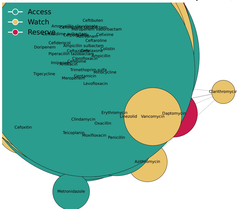
(a) Antibiotic co-resistance network (colored by AWaRe)
