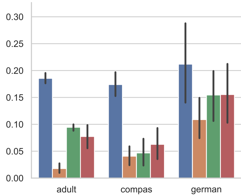
Statistical Parity
