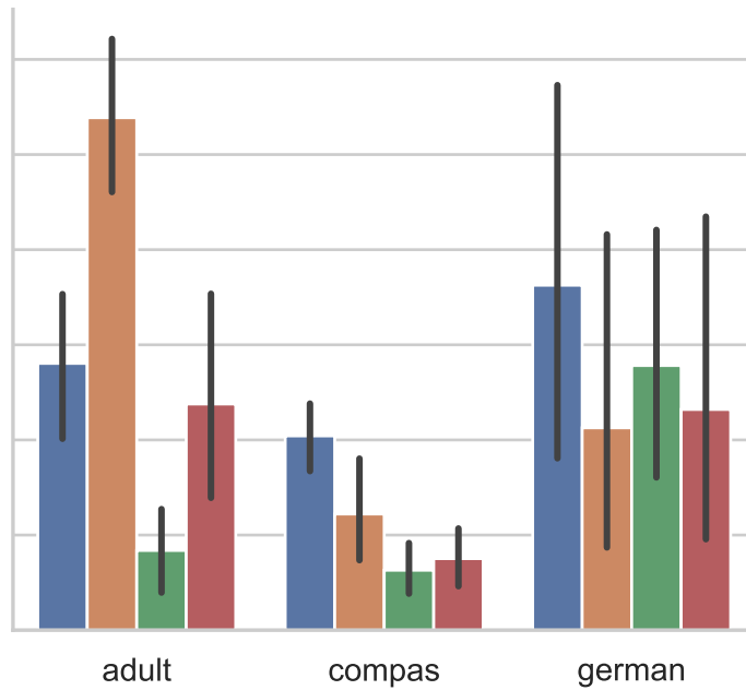
Equal Opportunity
