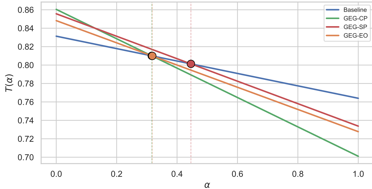
XGBoost
