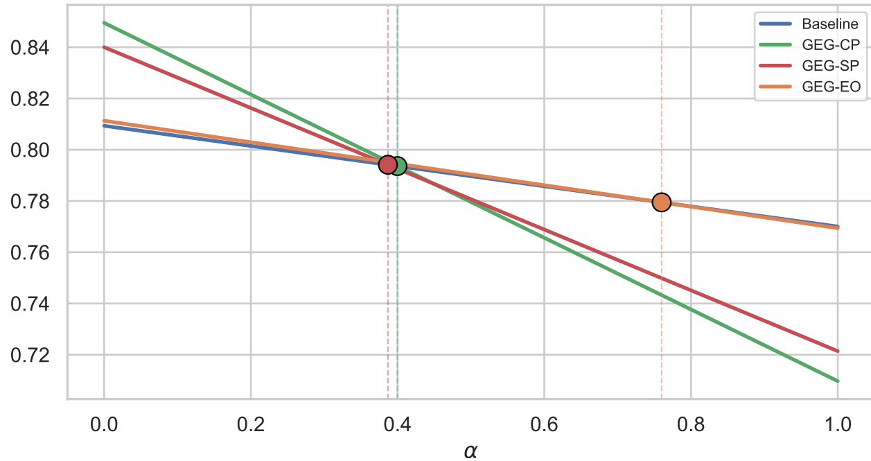
Random Forest
