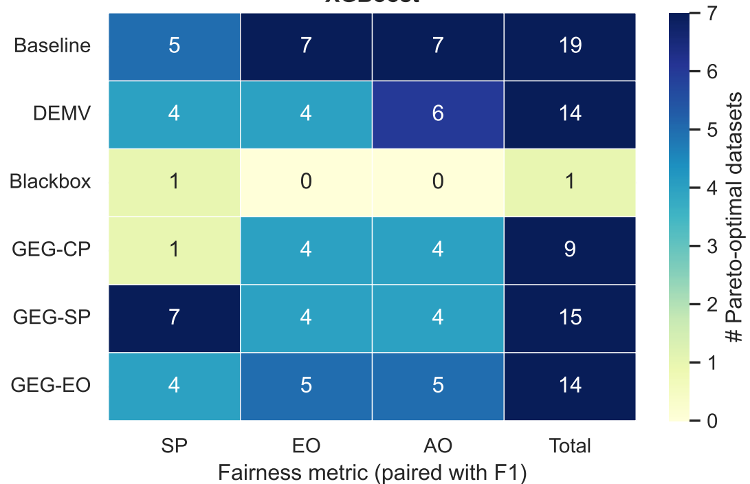
XGBoost
