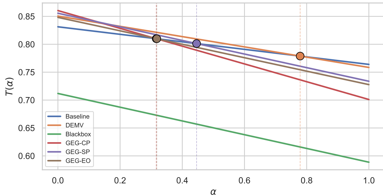
XGBoost
