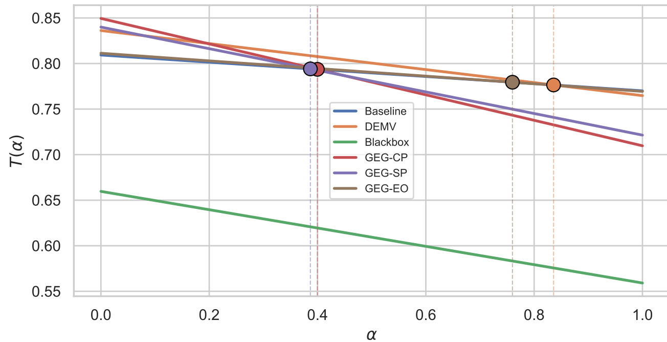
Random Forest
