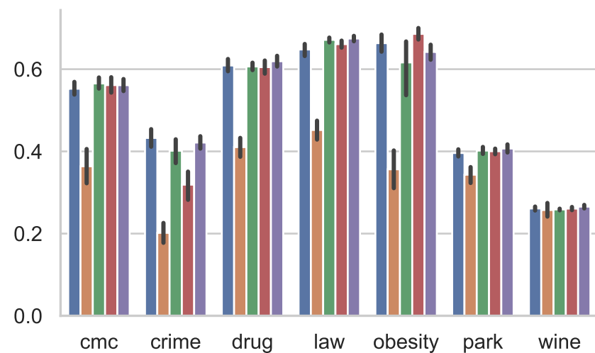
Recall
