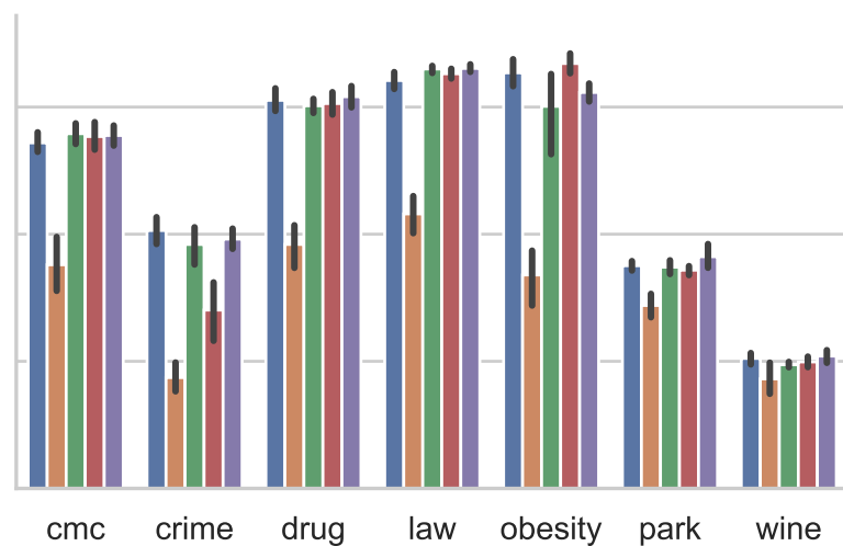
F1-score
