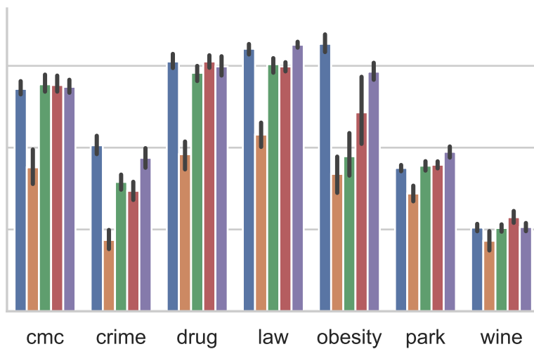
F1-score
