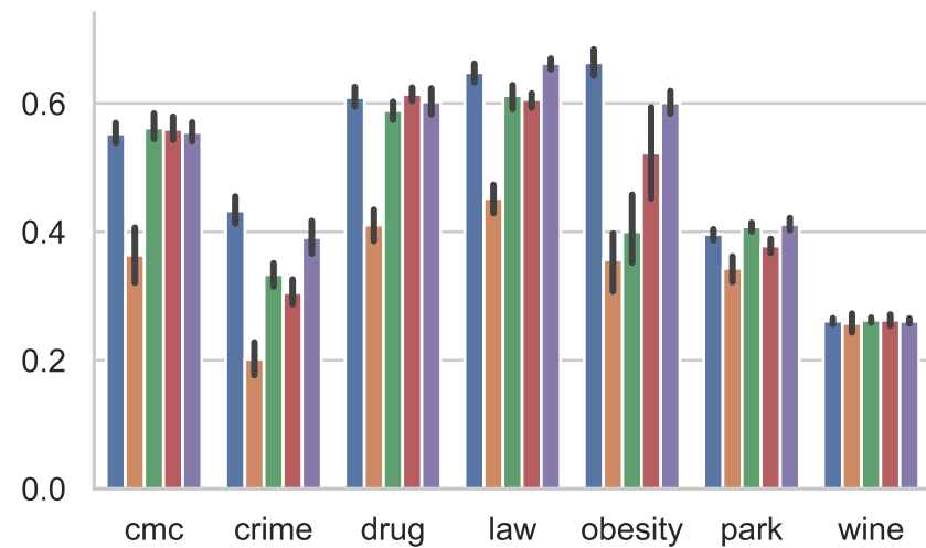
Recall
