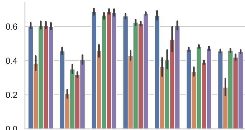
Accuracy
