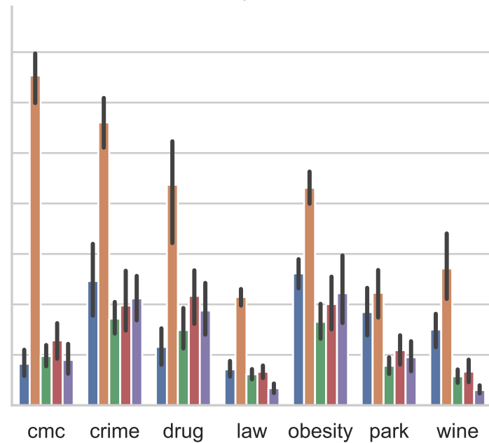
Average Odds
