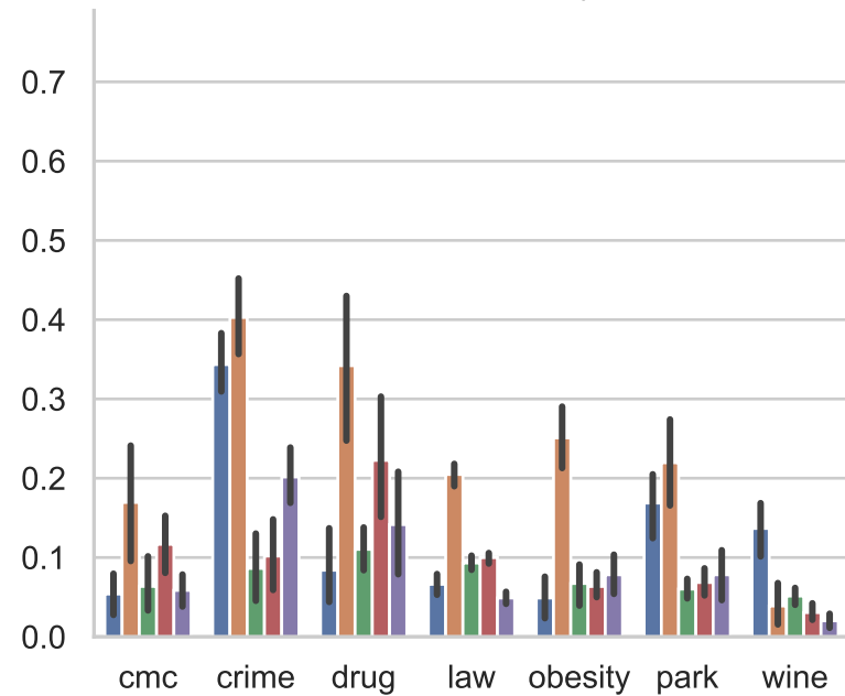
Statistical Parity
