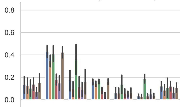
Random Forest | Statistical Parity
