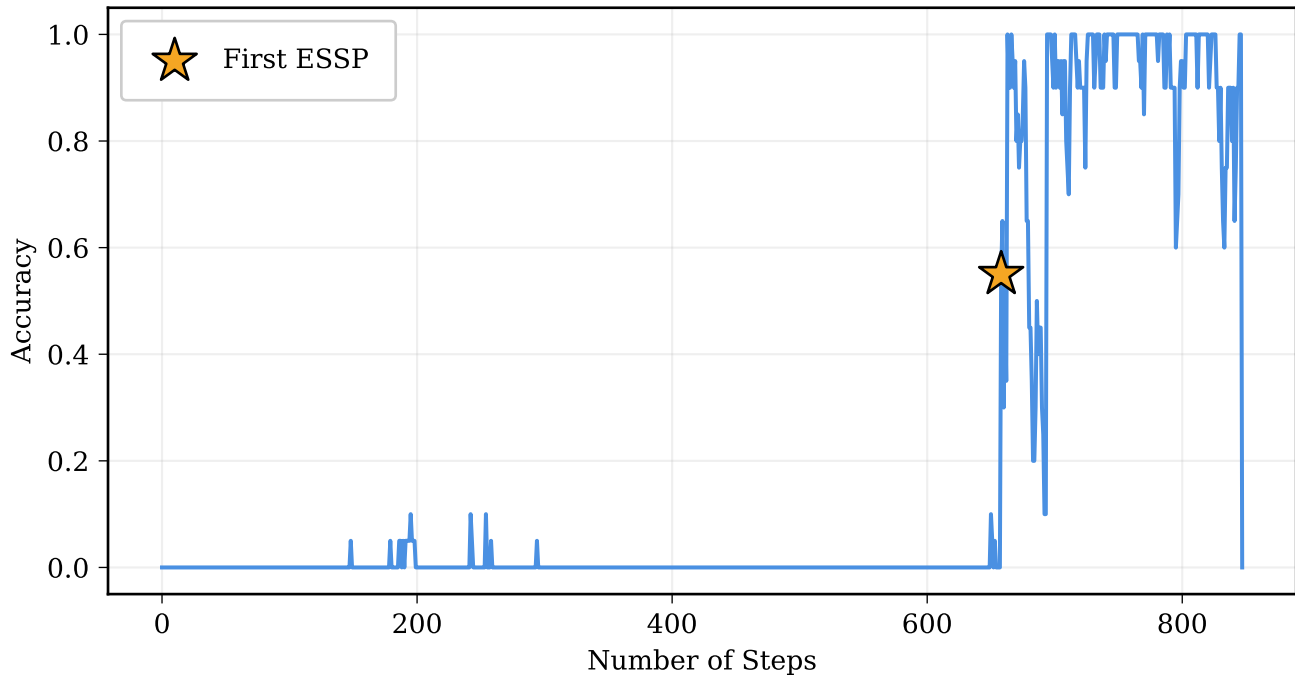
Early Stopping Success: Problem 0
