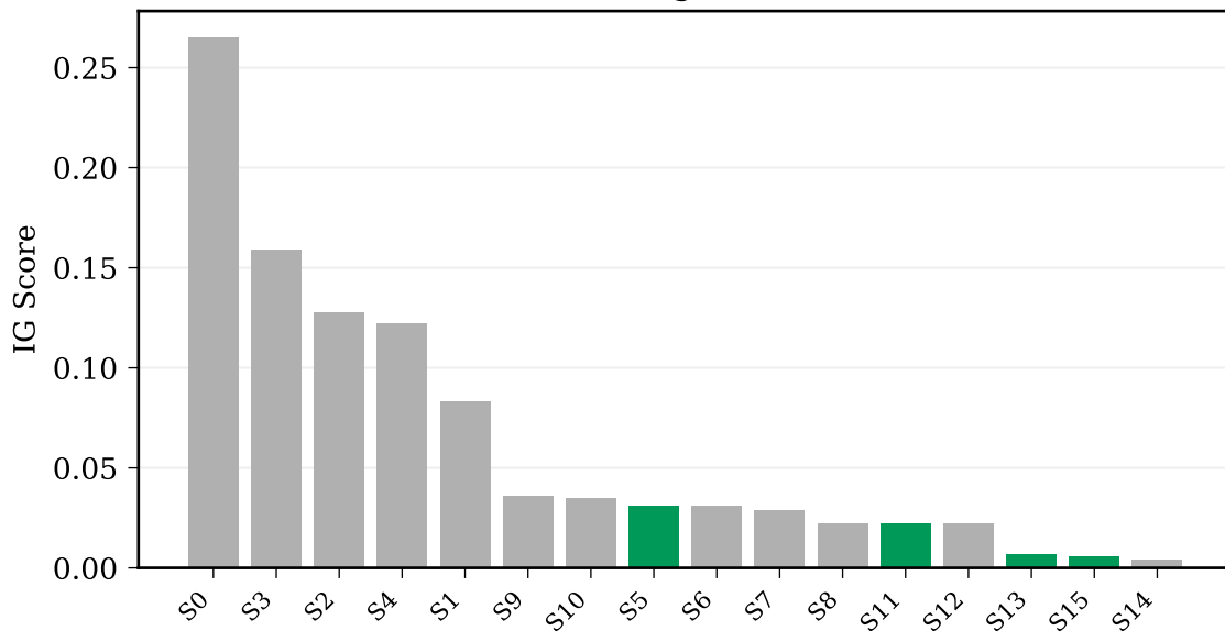
Problem 1: Integrated Gradients
