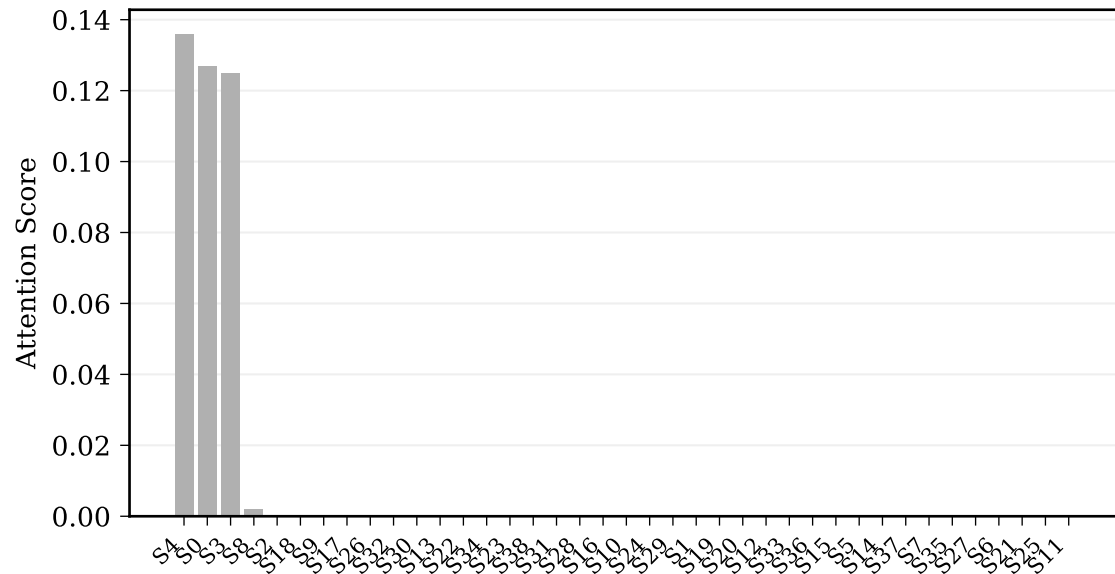
Problem 1: Attention
