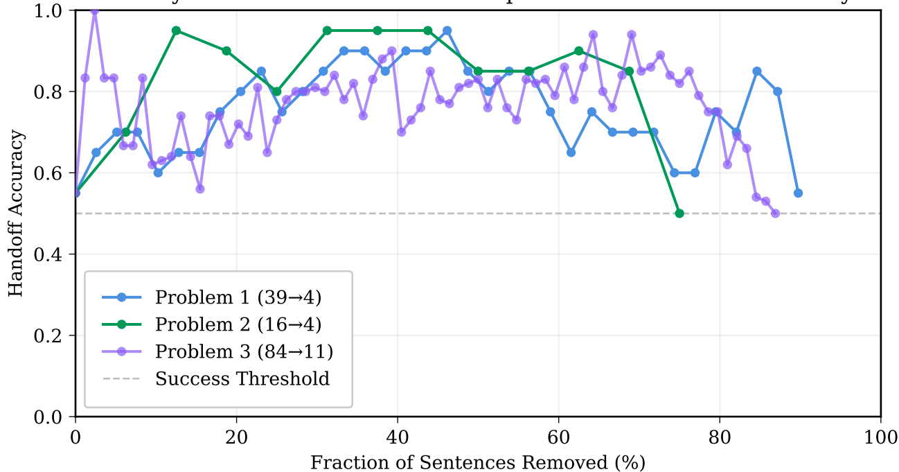
Greedy Backward Elimination: Compression vs. Transfer Accuracy
