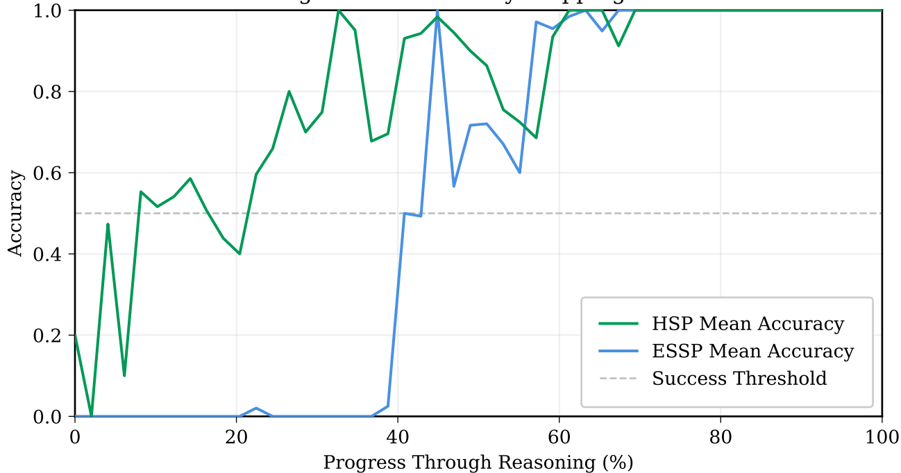
Average Handoff & Early Stopping Success
