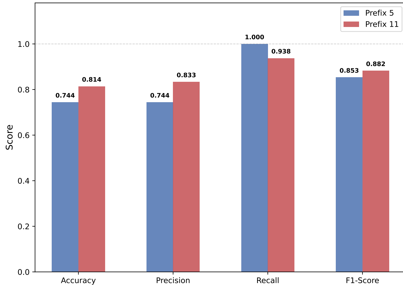
Decision Tree Prediction
