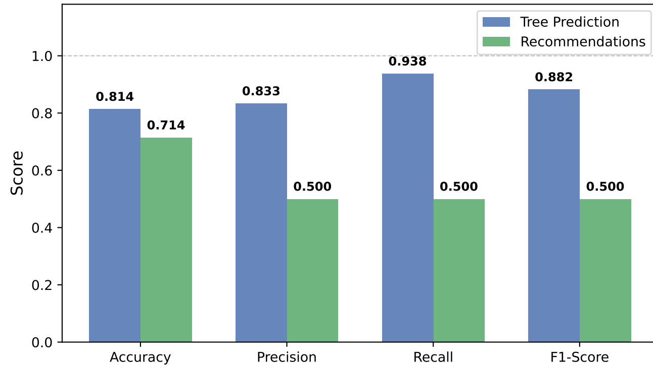
Tree Prediction vs Recommendation
