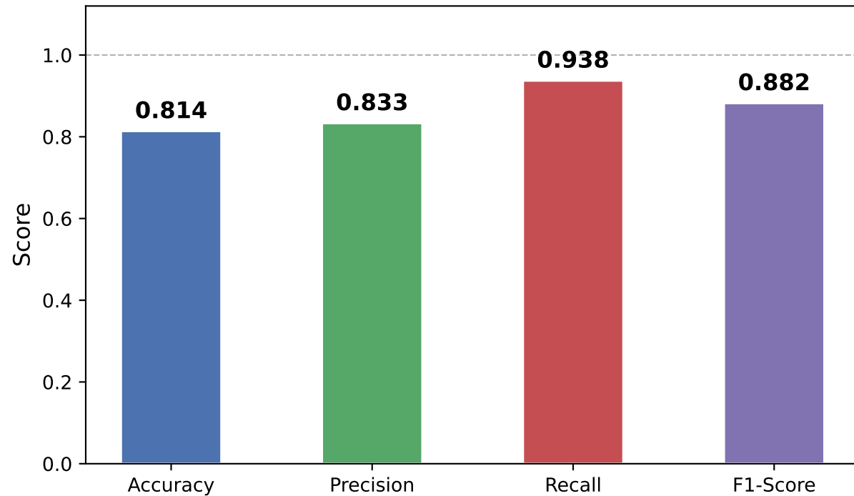
Performance Metrics
