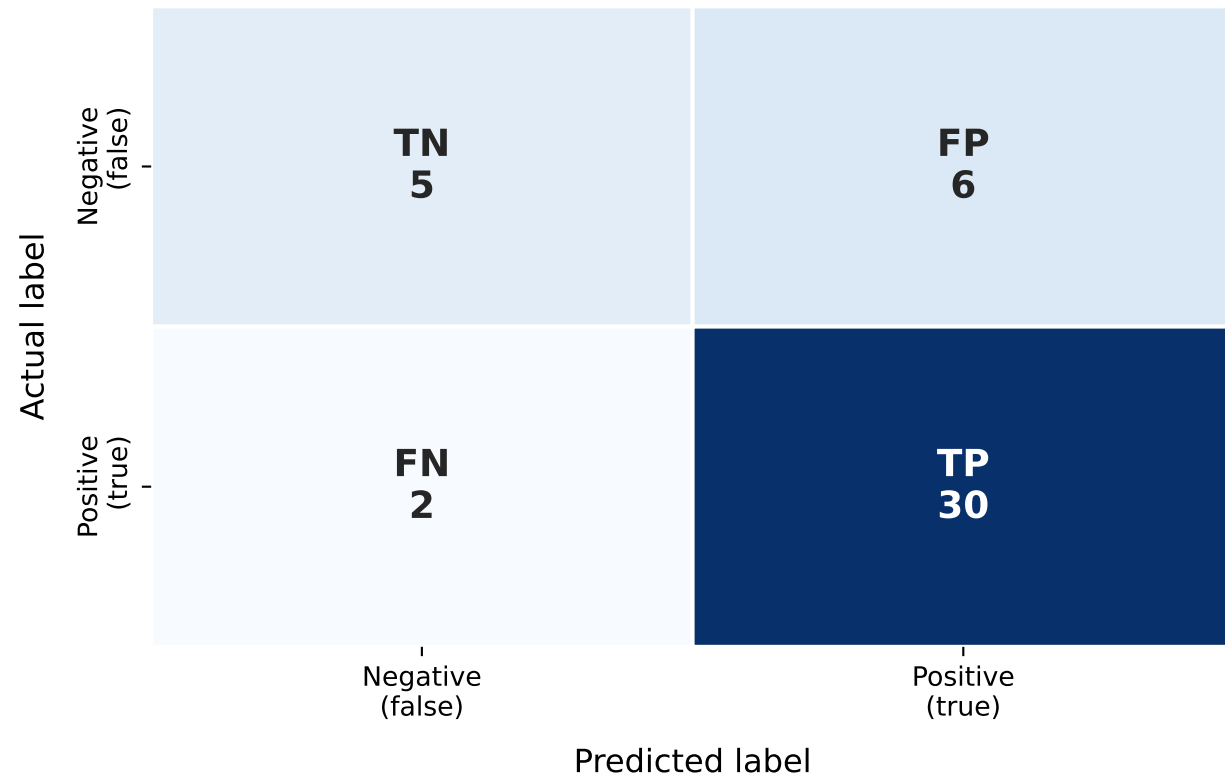
Confusion Matrix
