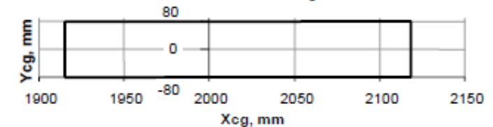
Lateral Balance diagram
