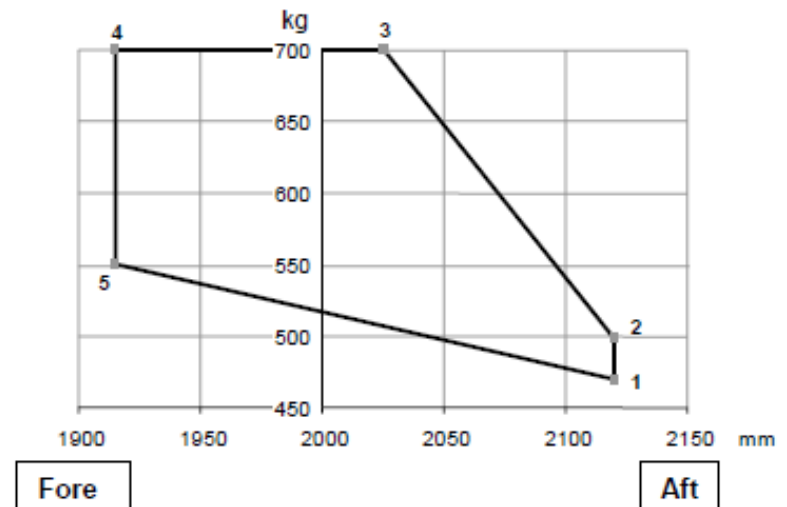
Longitudinal Weight and Balance diagram
