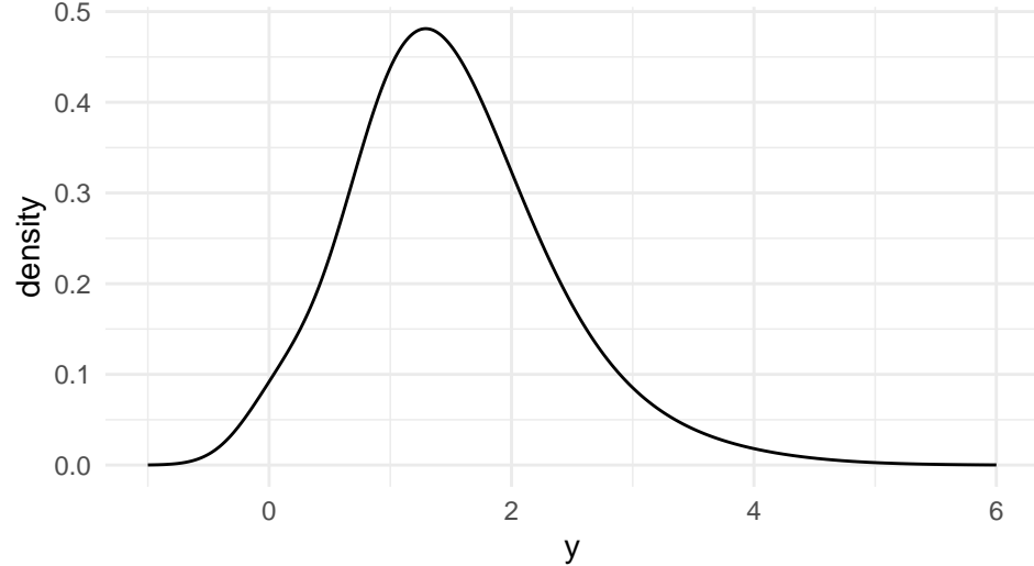
Moderate transmission (Beta) – Marginal Density of Y
