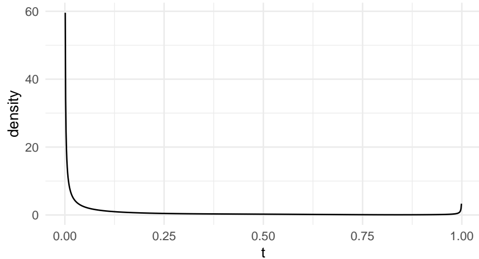
High transmission (Beta) – Density of T
