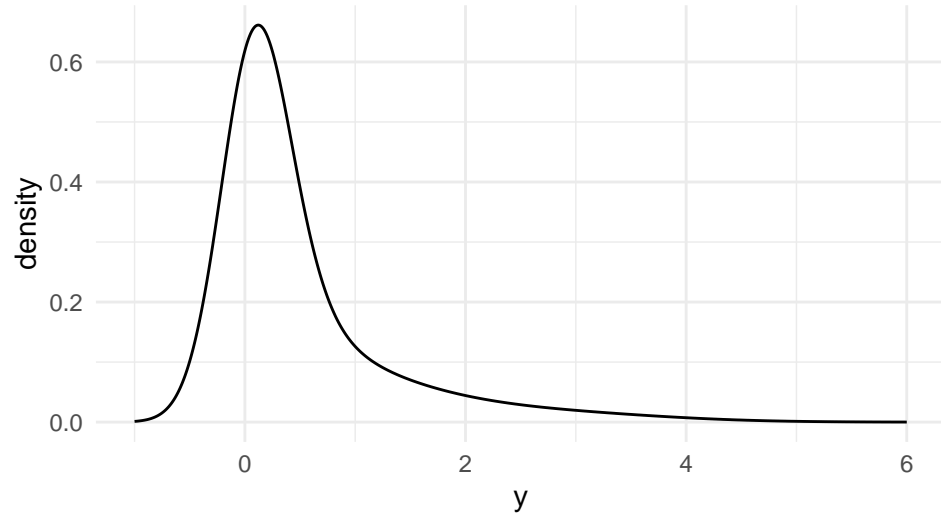
High transmission (Beta) – Marginal Density of Y
