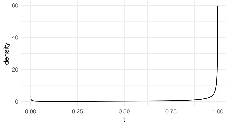
Moderate transmission (Beta) – Density of T
