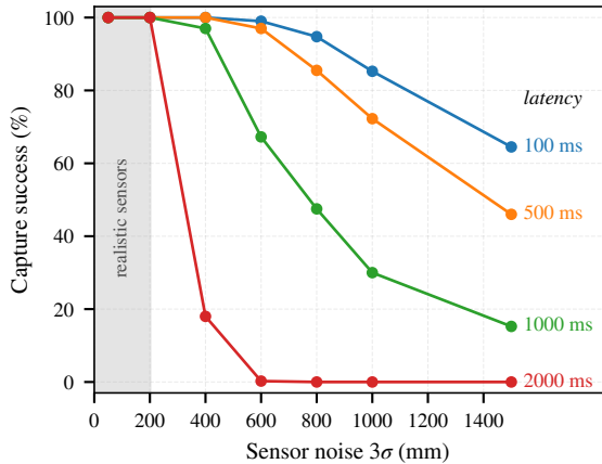
(b) Success versus sensor noise
