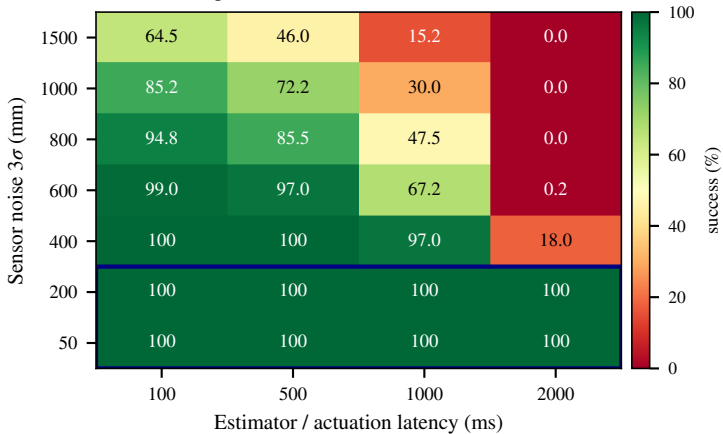
(a) Capture success (%); box: realistic sensors
