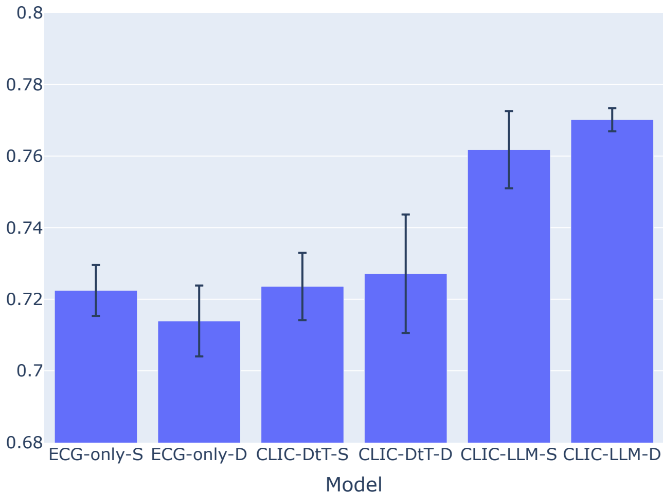
General Accuracy
