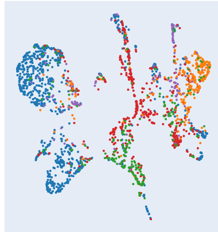
● STTC ● CD ● HYP CLIC-DtT (Silhouette: 0.1279)
