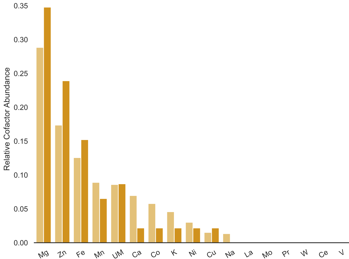
Test-organisms's cofactor usage relative to nearest neighbors
