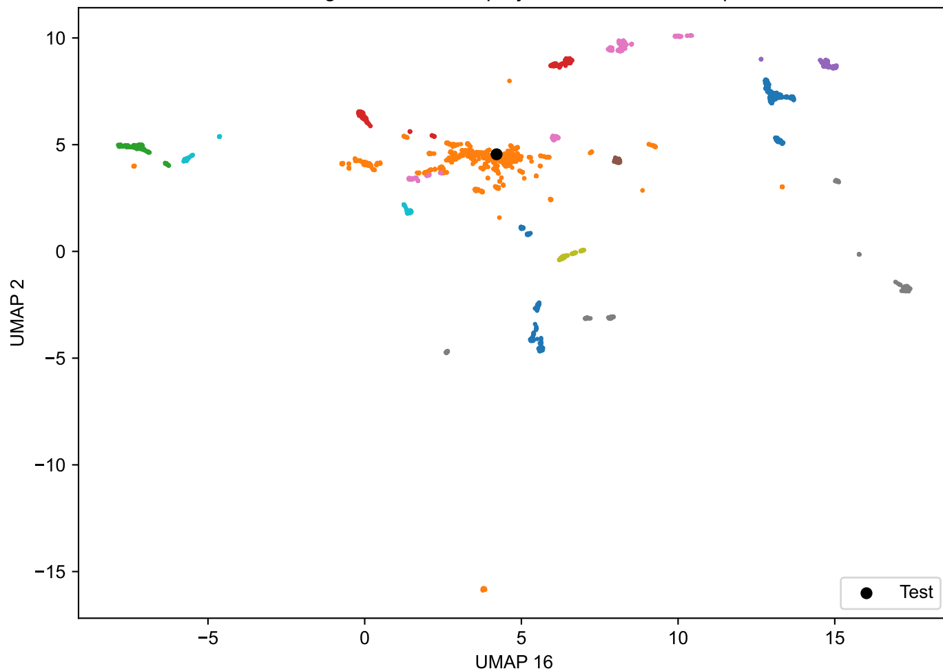
Test organism's UMAP projection in metabolic space
