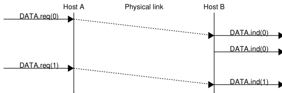
Figura 3.3: De-synchronization [1]
