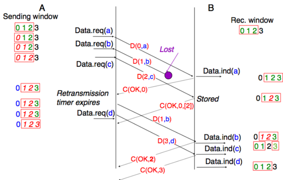
Figura 3.13: Selective repeat [1]
