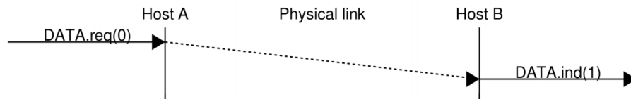
Figura 3.2: Bit flipping [1]
