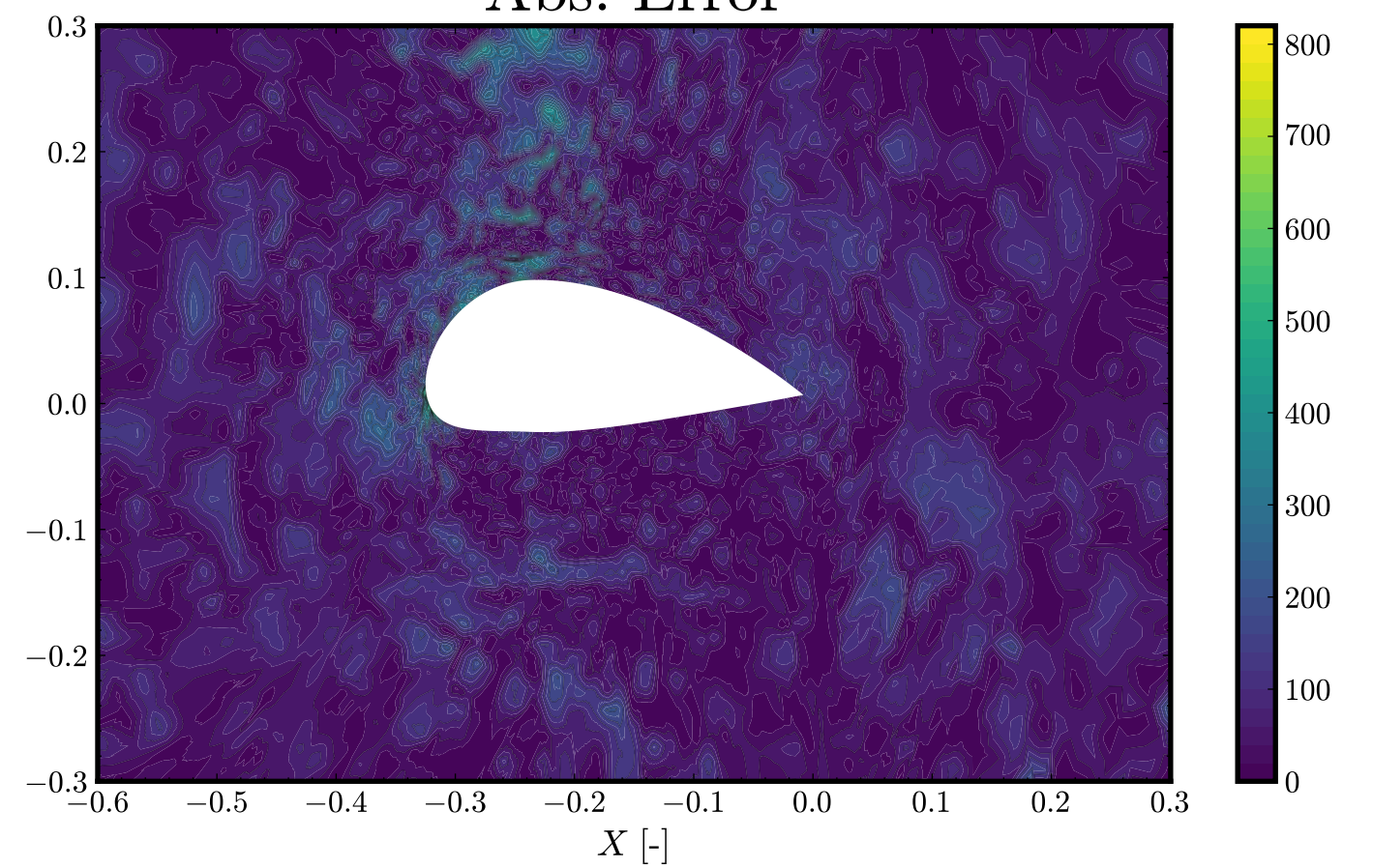
Abs. Error
