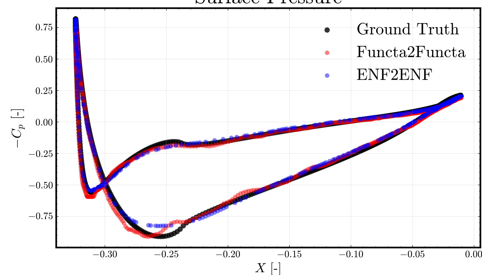
Surface Pressure
