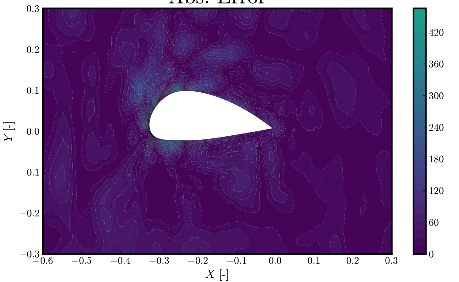
Abs. Error
