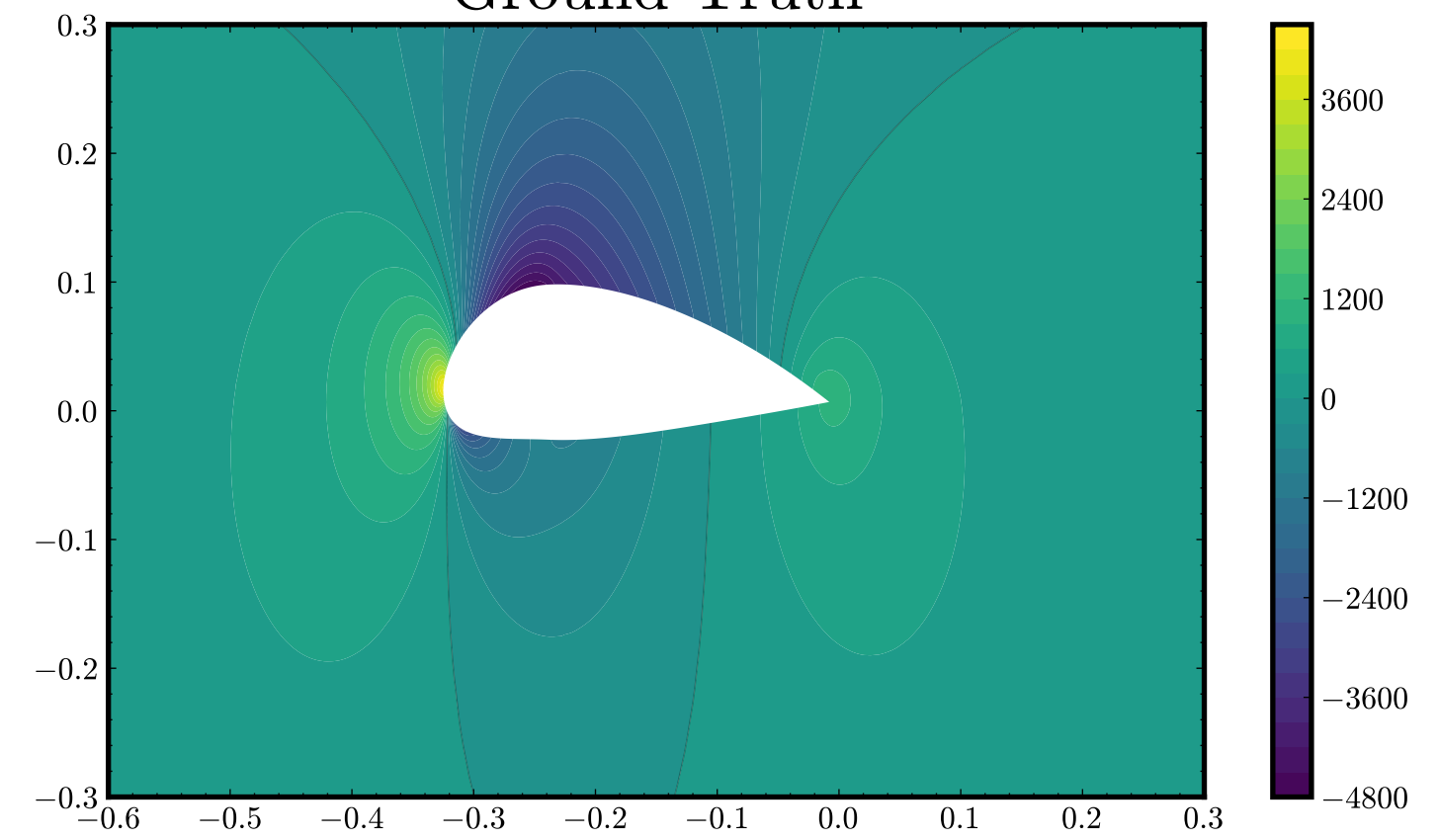
Surface Pressure
