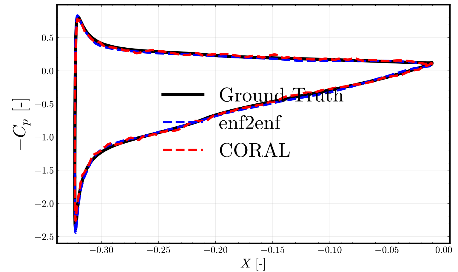
Surface Pressure
