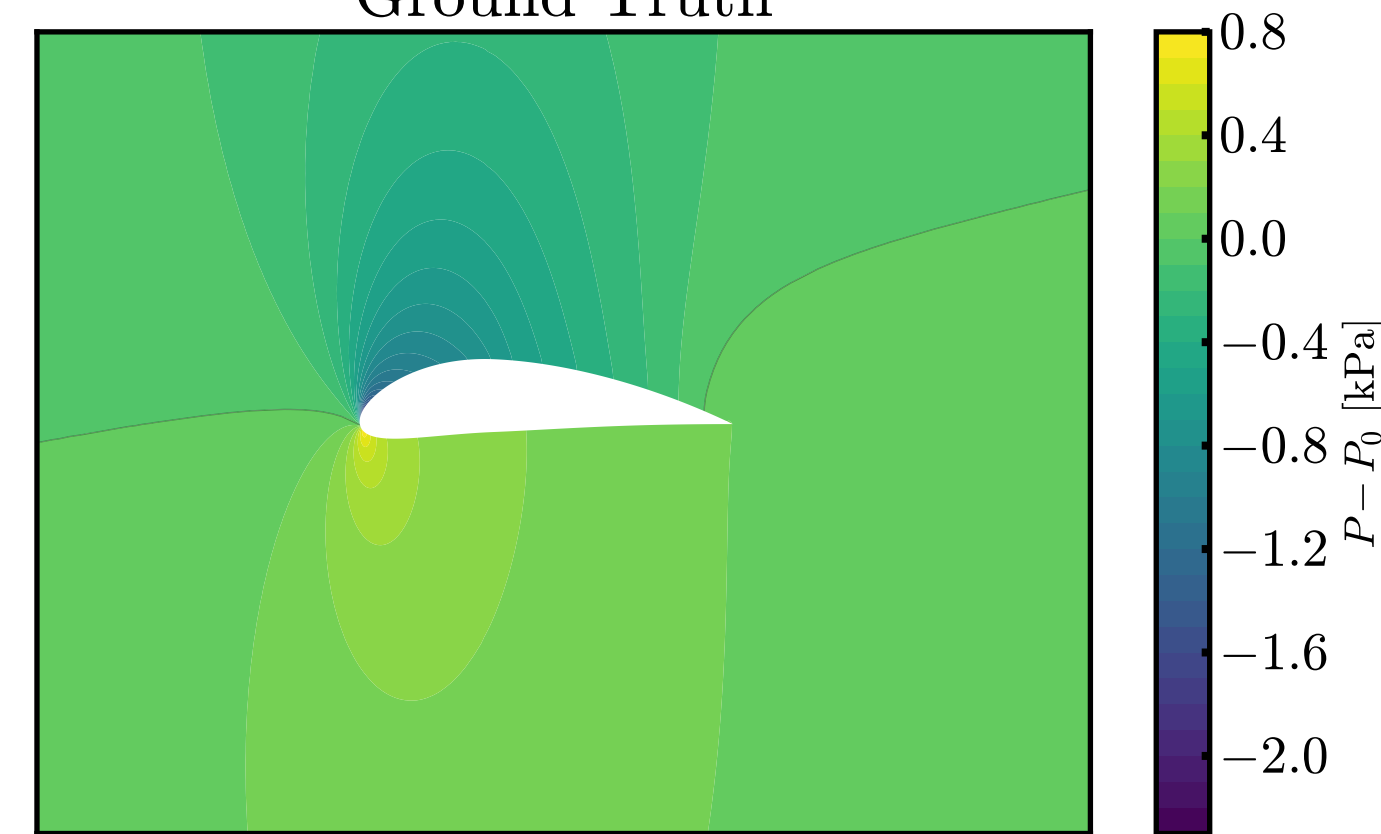
Surface Pressure
