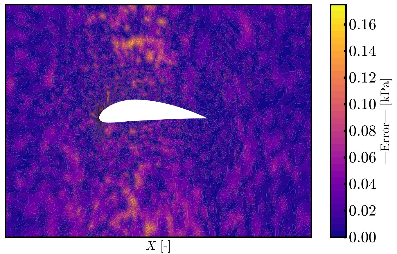
Abs. Error
