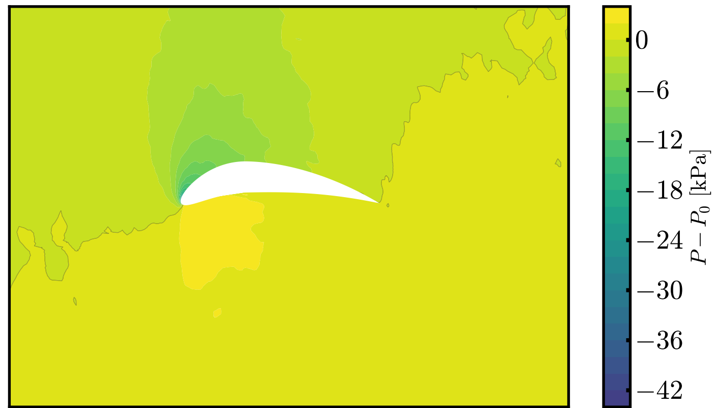
CORAL
