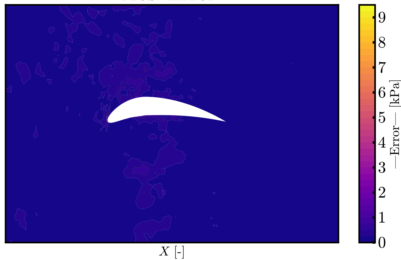
Abs. Error
