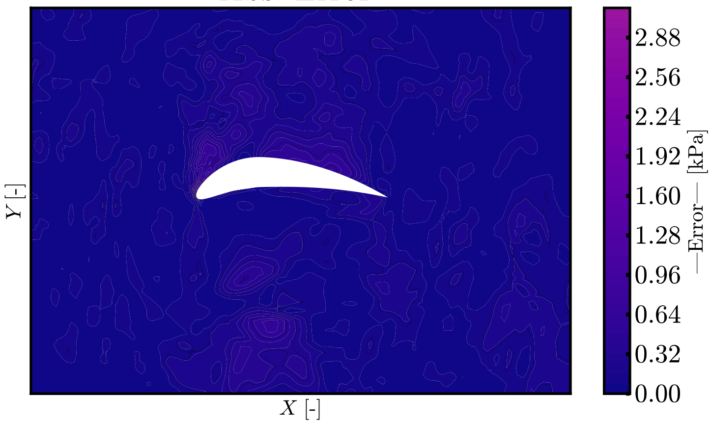
Abs. Error
