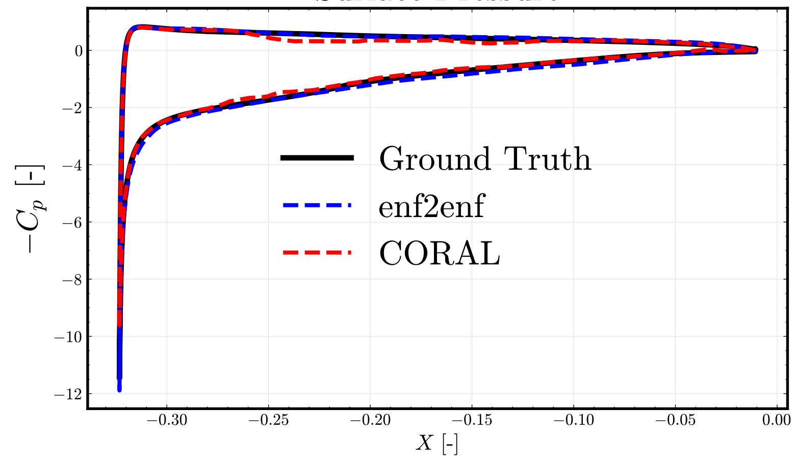
Surface Pressure
