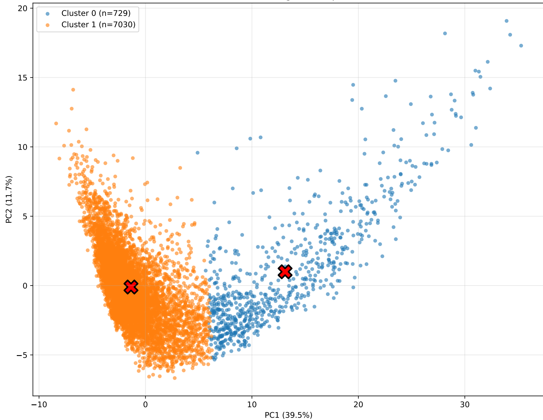
K=2 clustering in PCA space
