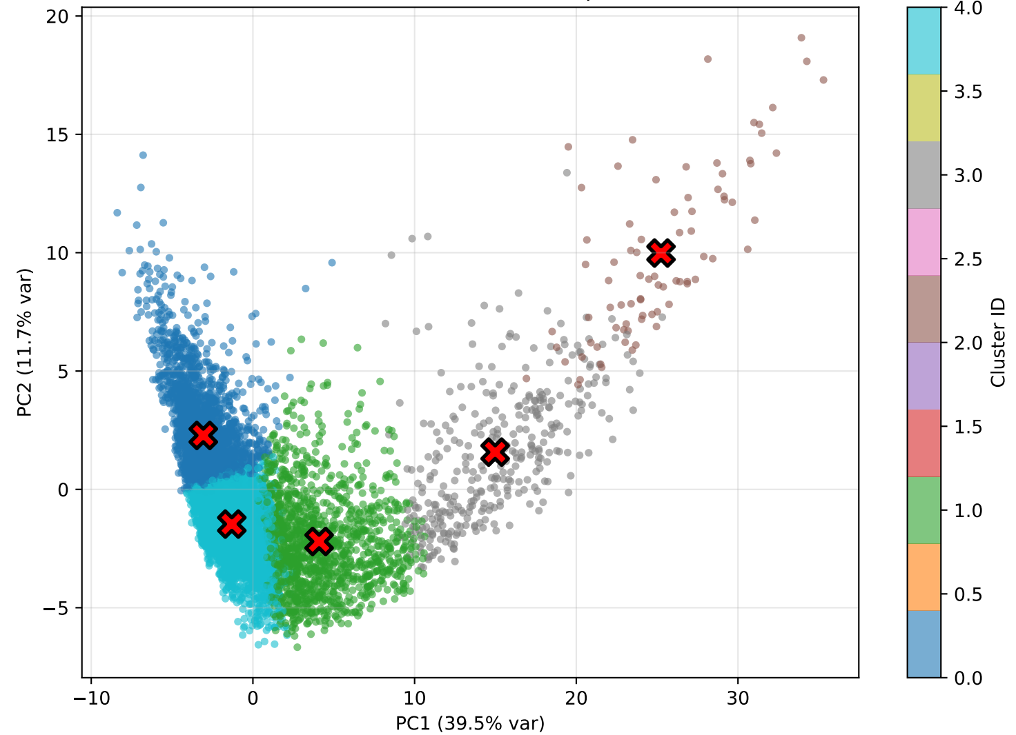
K-means K=5 in 2D PCA space
