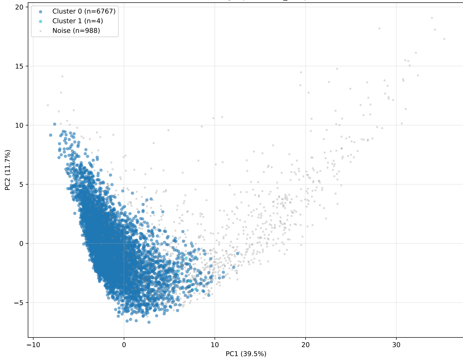
DBSCAN clustering (eps=5, min_samples=5)
