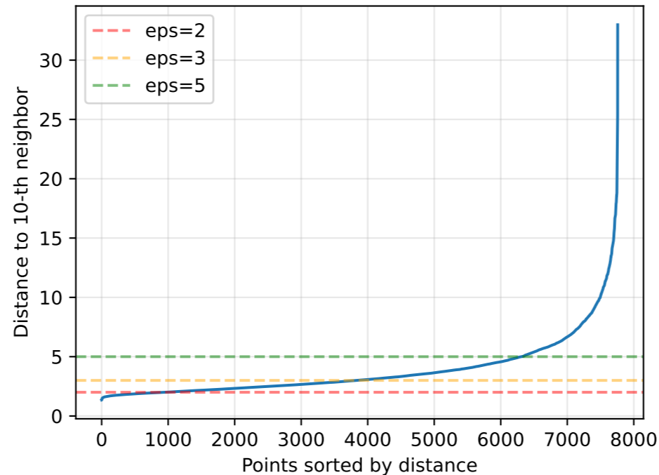
k=10 nearest neighbor
