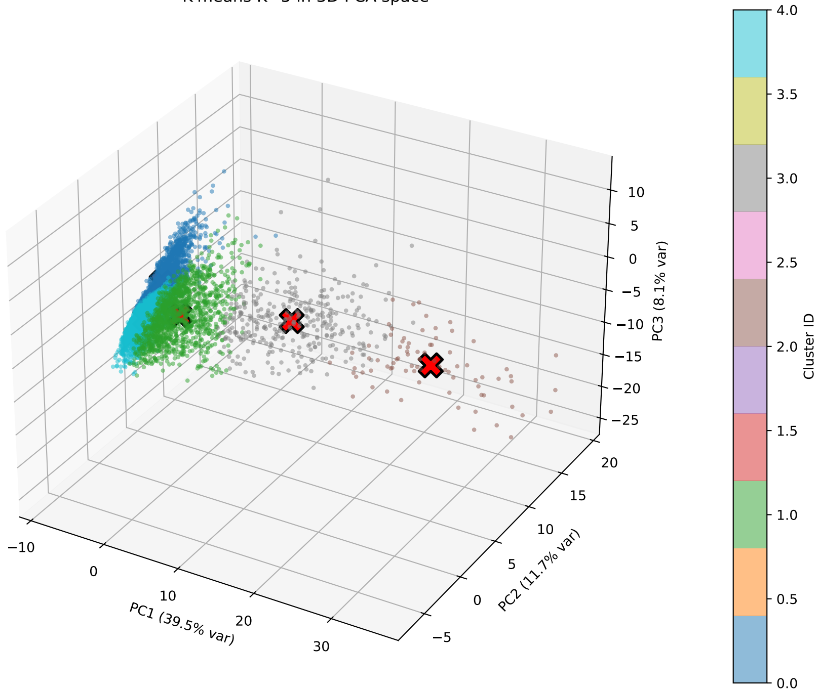
K-means K=5 in 3D PCA space
