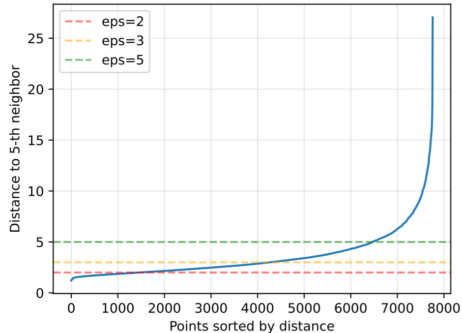
k=5 nearest neighbor
