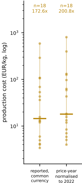
a1 full literature cohort
