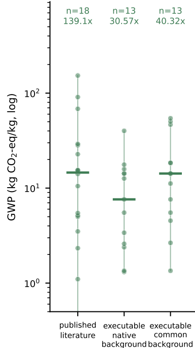
b GWP populations
