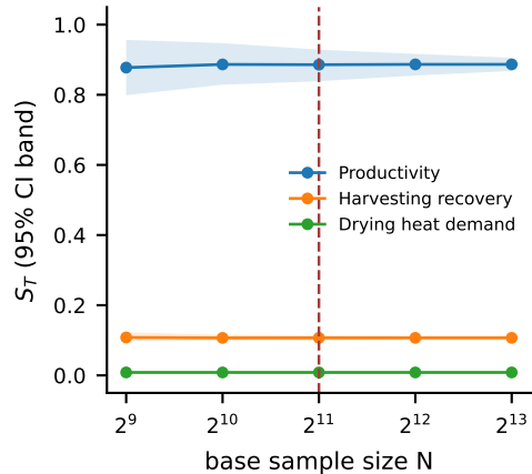
Open raceway pond (Chlorella)
