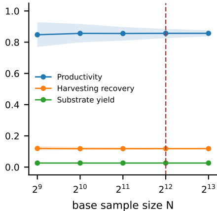
Heterotrophic fermenter (Schizochytrium)
