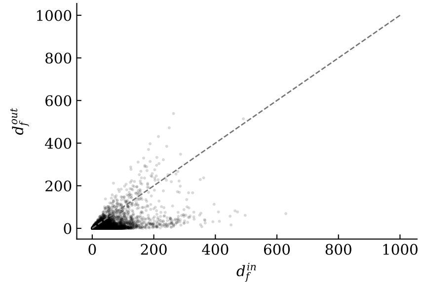
d^{in} vs d^{out} (45° line)
