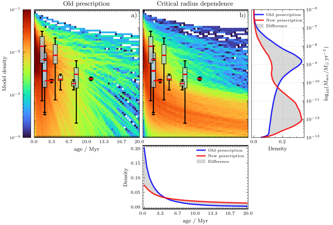
Figure 5. Mass accretion rate as a function of time for the old prescription (panel a) and the critical radius criteria (panel b). The corner plots show the density distribution in the accretion rates and disc age, and the difference as a gray shadow region. The disc observed properties (Manara et al. 2023; Thanathibodee et al. 2022) are overplotted as box plots.
