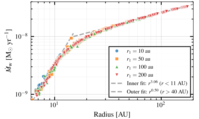
Figure 2. Cumulative mass loss rate as a function of radius for different critical radii.
