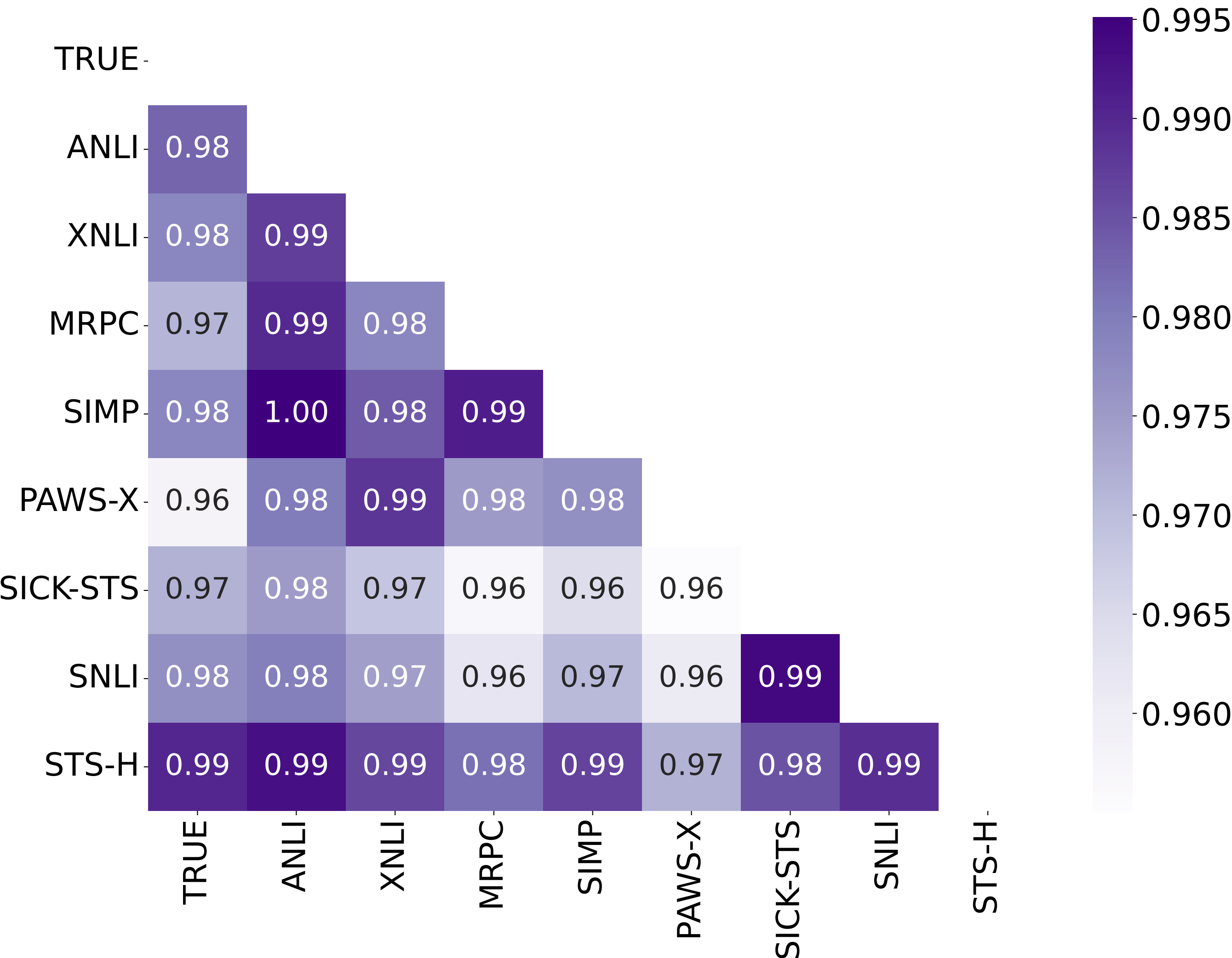
Dataset Similarity Matrix using multilingual-e5-large-instruct
