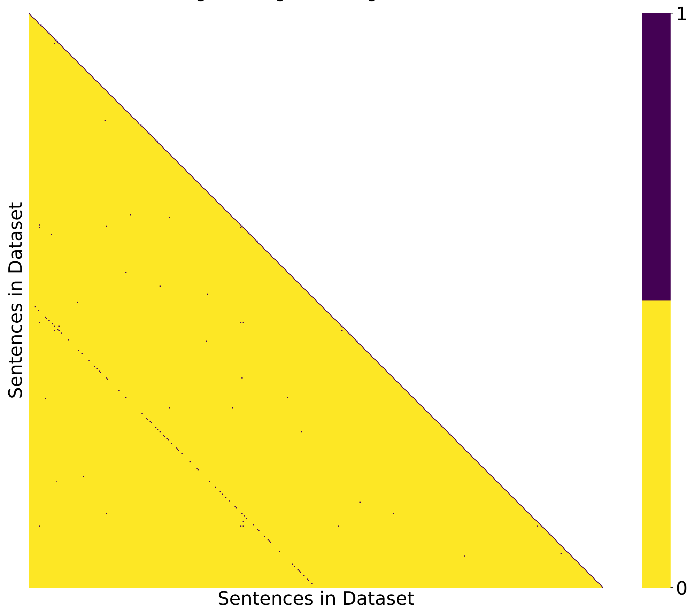
Predictions for STSB using multilingual-e5-large-instruct (Thresholded at 0.95)
