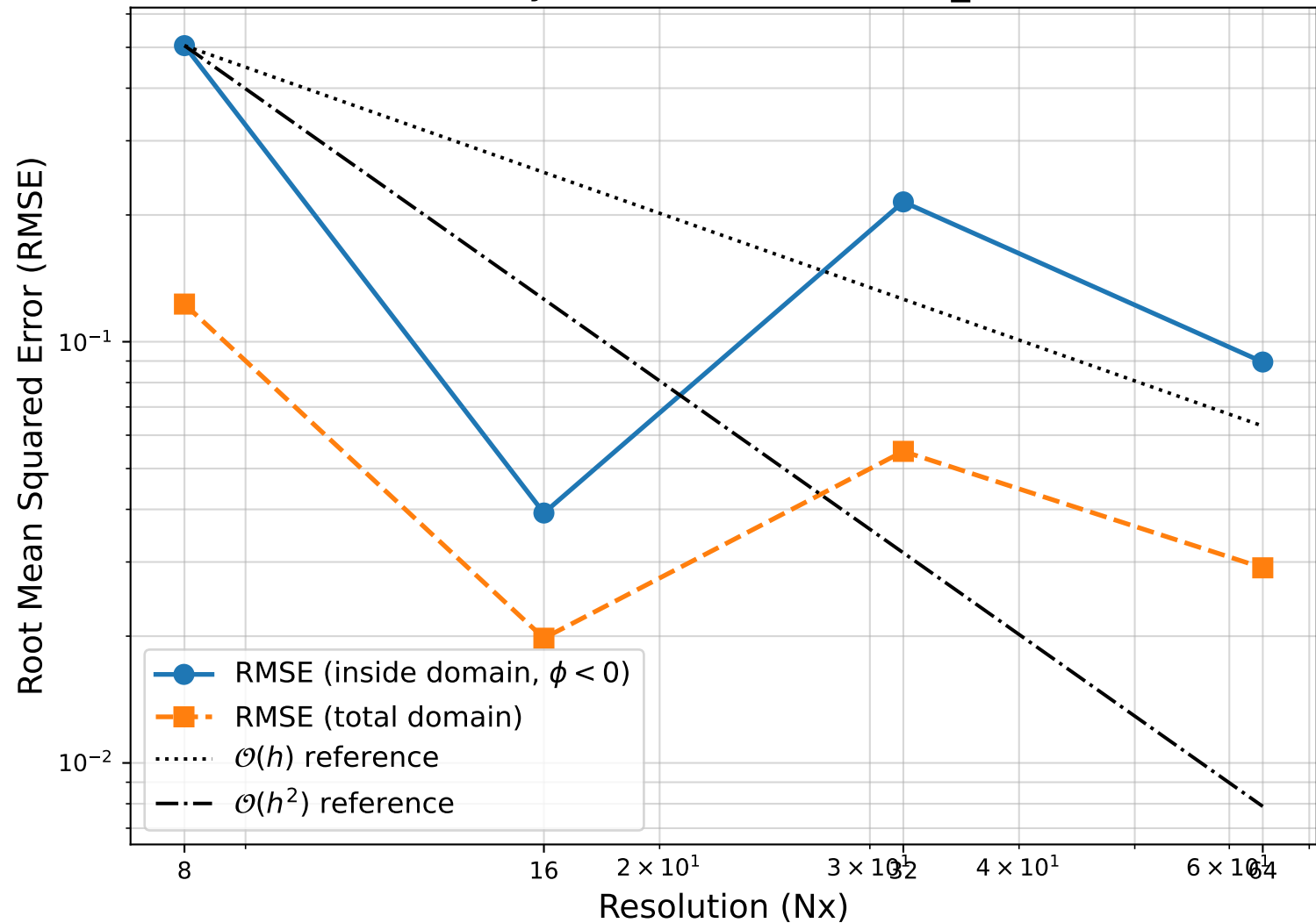
RMSE vs System Resolution (star_Robin3)
