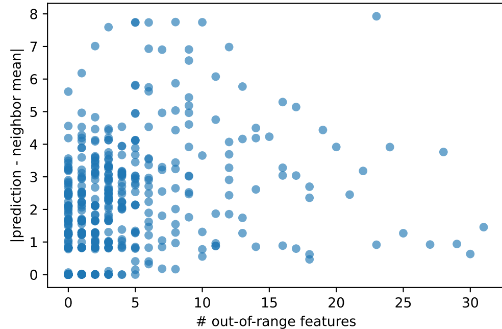
Out-of-range burden vs local deviation
