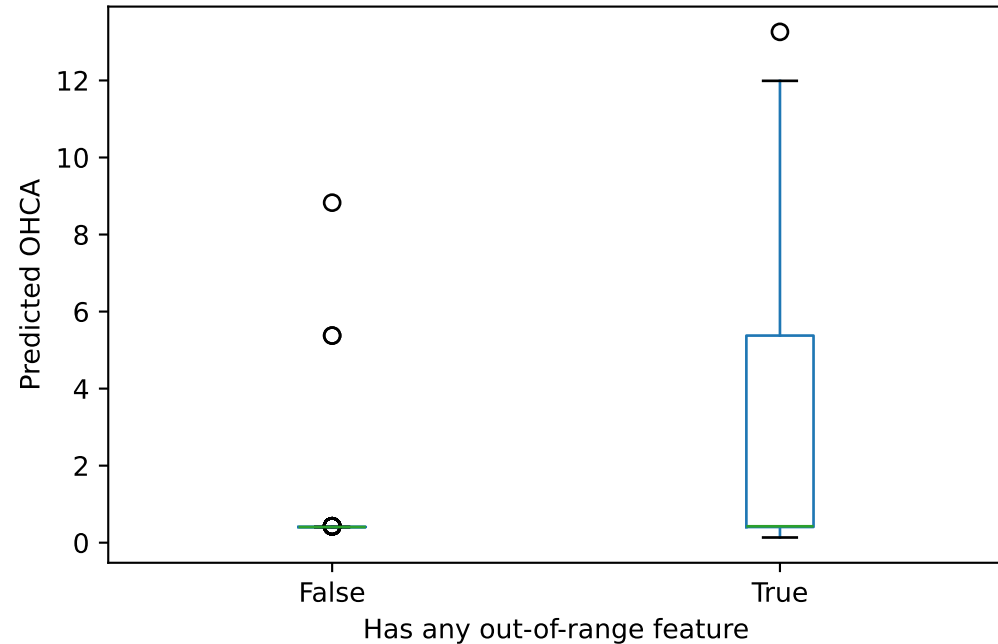
Prediction by out-of-range status
