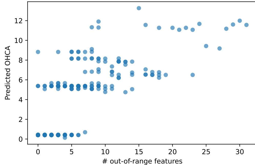
Out-of-range burden vs prediction
