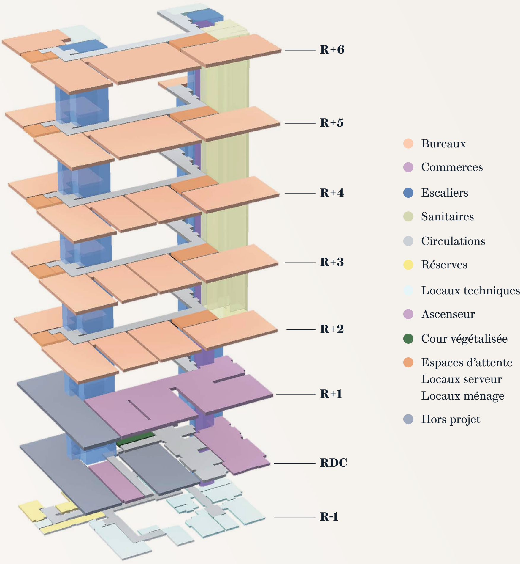
Stacking plan
