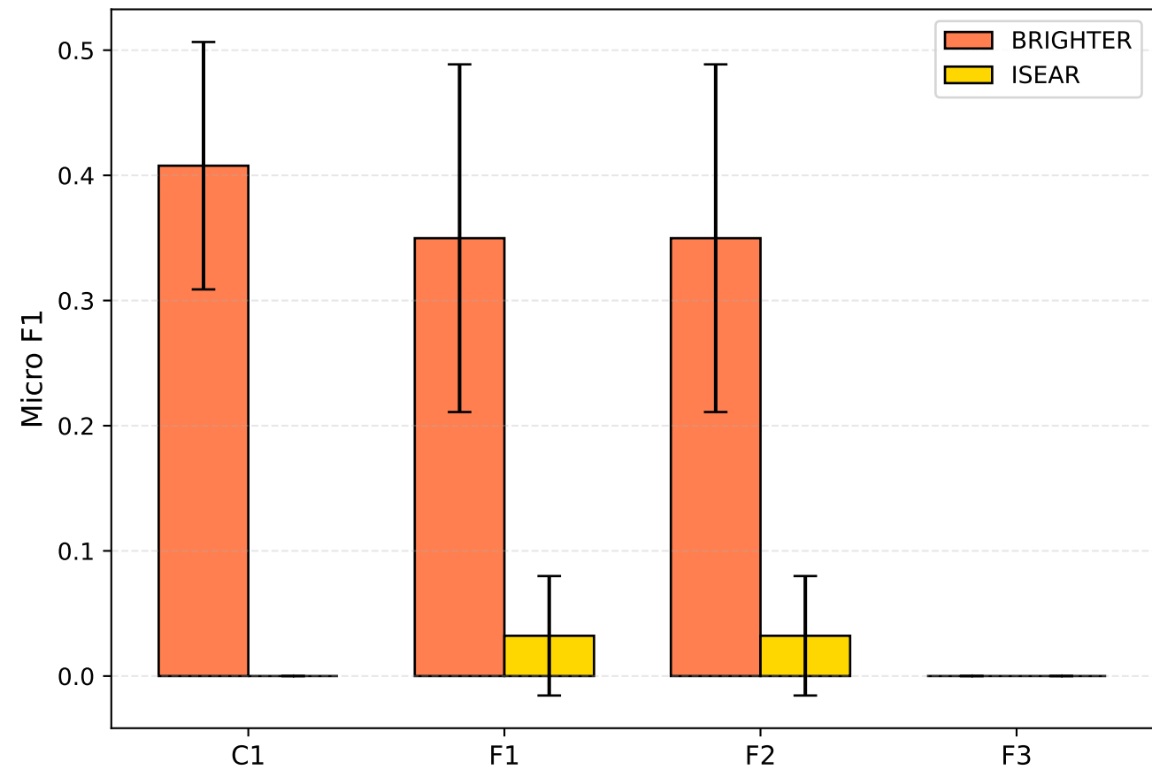
(b) Micro F1: BRIGHTER vs ISEAR
