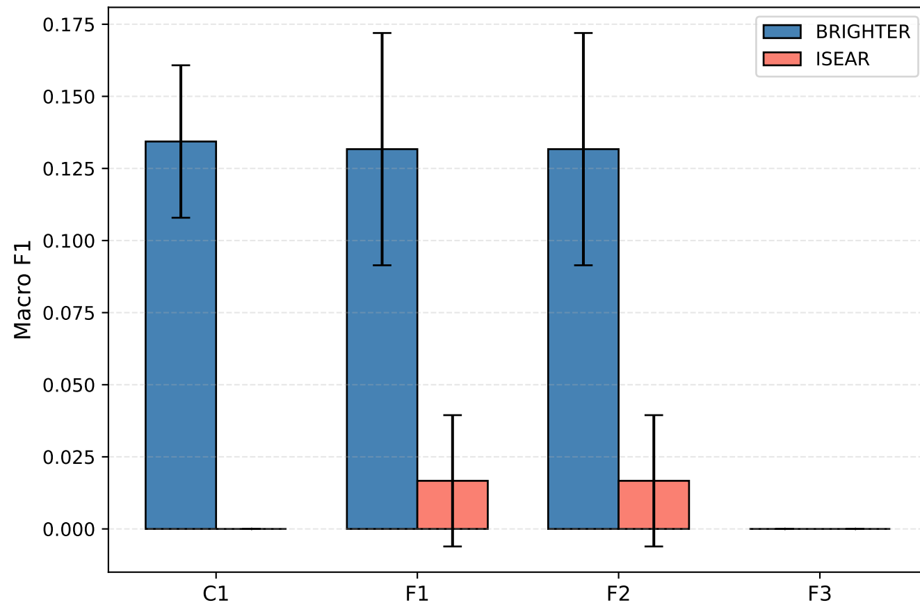
(a) Macro F1: BRIGHTER vs ISEAR
