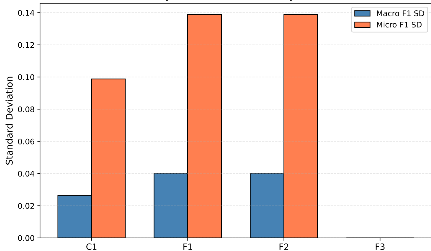
Seed-level Stability: Standard Deviation by Method (BRIGHTER)
