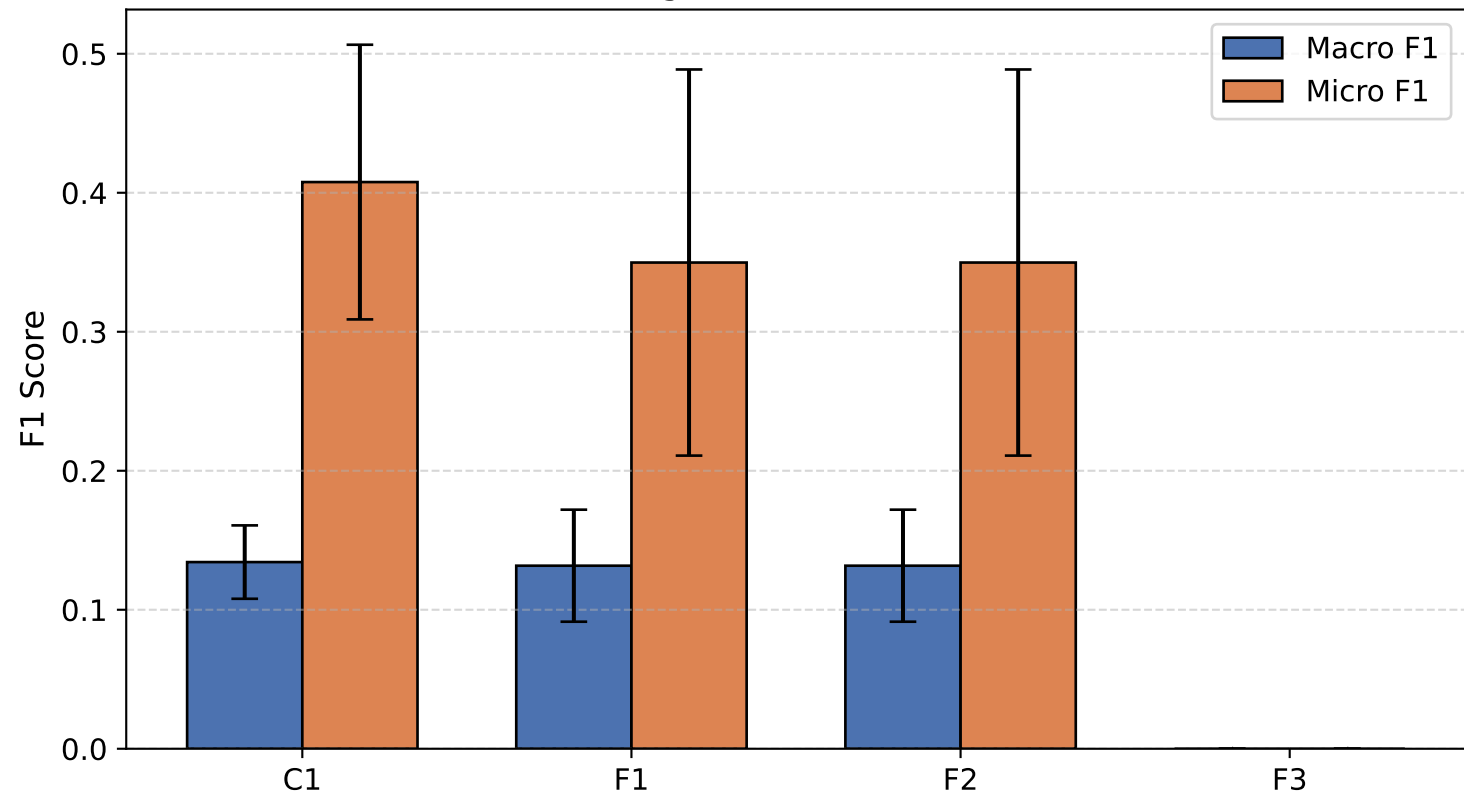
BRIGHTER English: C1/F1/F2/F3 (10 seeds)
