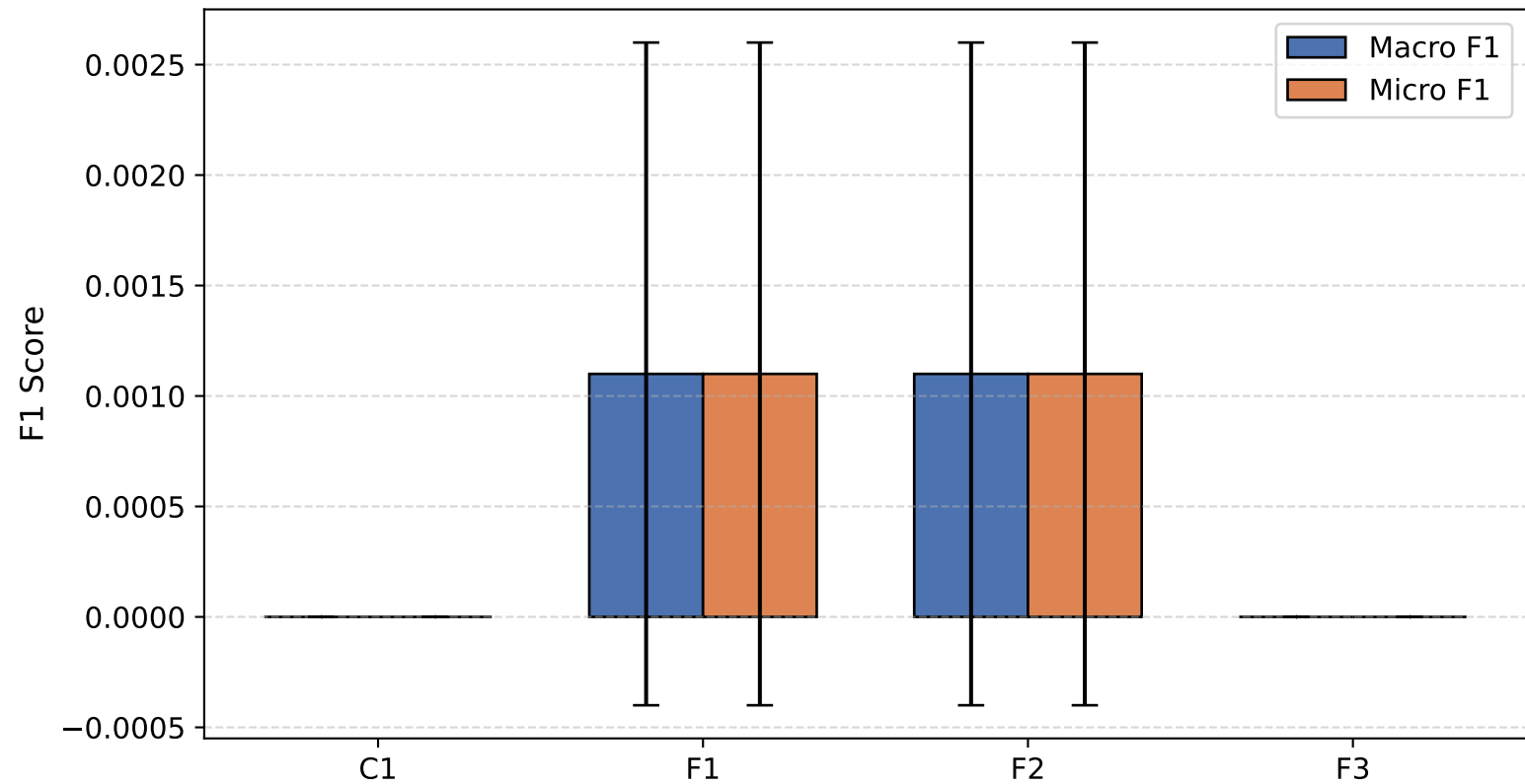
GoEmotions (Filtered): C1/F1/F2/F3 (5 seeds)
