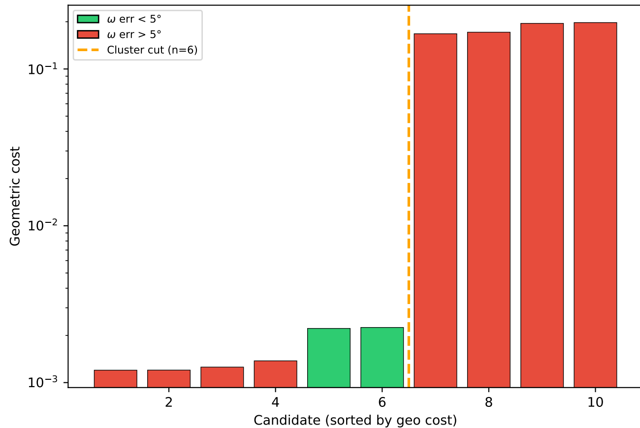
Seed 93: Geometric refinement — cluster detection
