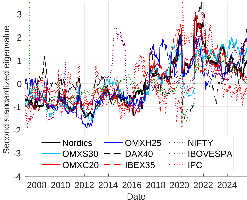
Second standardized eigenvalues
