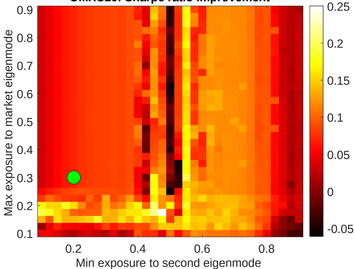
OMXC20: Sharpe ratio improvement
