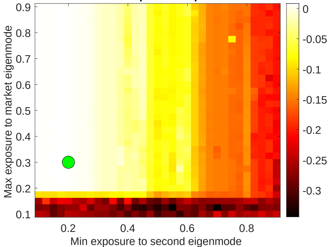
OMXS30: Sharpe ratio improvement
